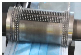
压花轮机构 Press and welding mechanism
